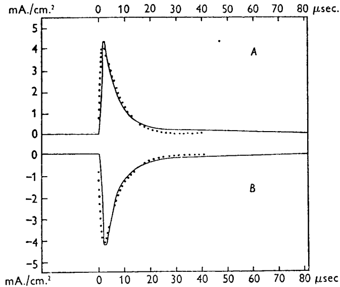
Fig. 16. Current through capacitive element of membrane during a voltage clamp. Abcissa: time in \mu\text{sec} . Ordinate: membrane current density ( \text{mA./cm.}^2 ) with inward current taken as positive. At t=0 the potential difference between external and internal electrodes was displaced +40 mV. in curve A or -40 mV. in curve B. The continuous curves were traced from experimental records. The dotted curves were calculated according to the equation
