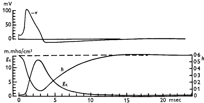
Fig. 19. Numerical solution of eqn. (26) for initial depolarization of 15 mV and temperature of 6° C. Upper curve: membrane potential, as in Fig. 13. Lower curves show time course of g_K and h during action potential and refractory period.
