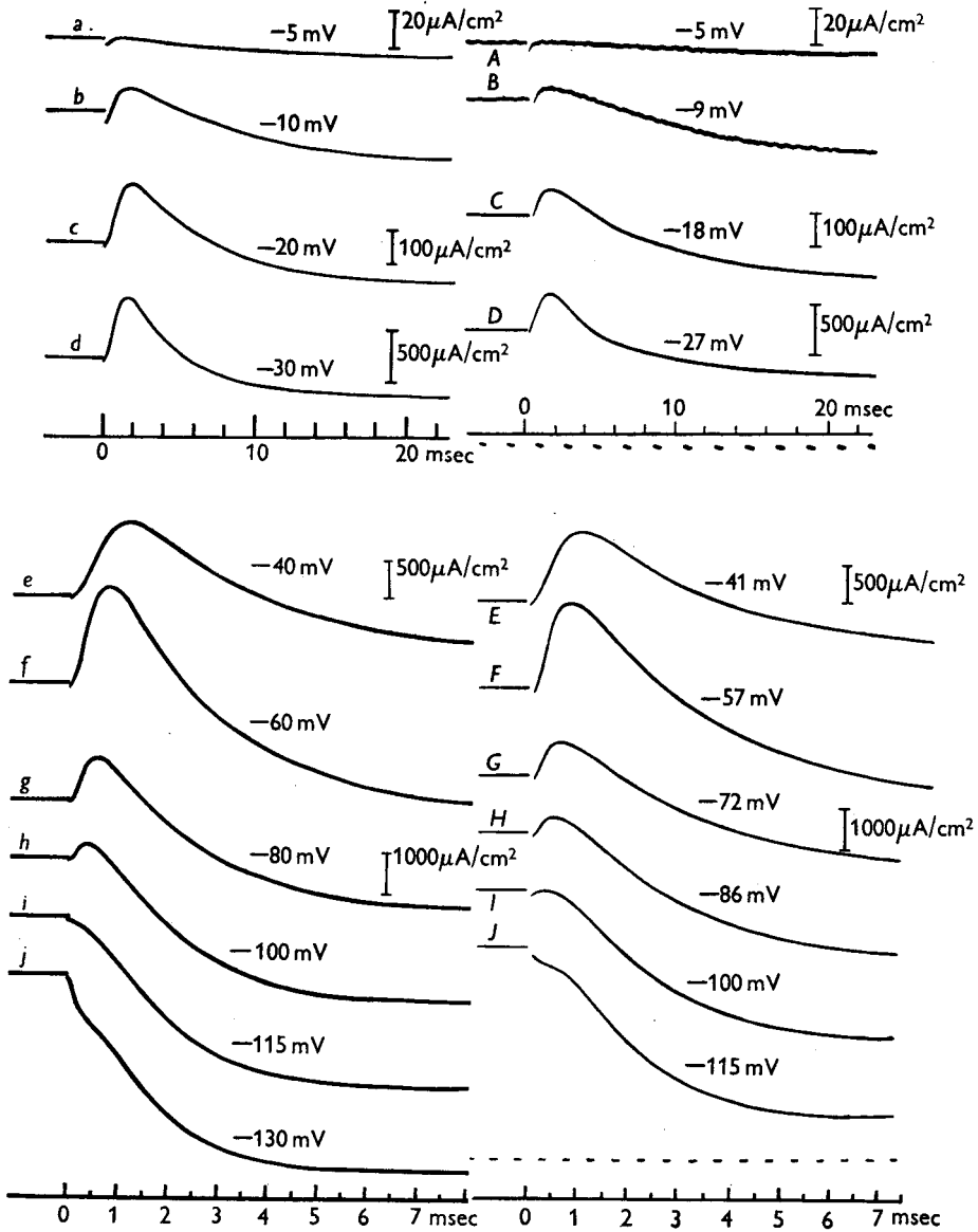
Fig. 11. Left-hand column: time course of membrane current during voltage clamp, calculated for temperature of 4° C from eqn. (26) and subsidiaries and plotted on the same scale as the experimental curves in the right-hand column. Right-hand column: observed time course of membrane currents during voltage clamp. Axon 31 at 4° C; compensated feedback. The time scale changes between d , D and e , E . The current scale changes after b , B ; c , C ; d , D and f , F .
