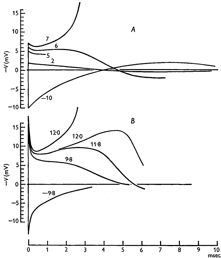
Fig. 21. A , numerical solutions of eqn. (26) for 6° C. The numbers attached to the curves give the initial depolarization in mV (also the quantity of charge applied in m\mu\text{coulomb/cm}^2 ). B , response of nerve membrane at 6° C to short shocks; the numbers show the charge applied in m\mu\text{coulomb/cm}^2 . The curves have been replotted from records taken at low amplification and a relatively high time-base speed.
