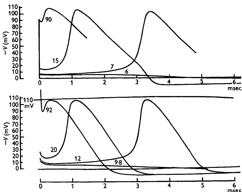
Fig. 12. Upper family: solutions of eqn. (26) for initial depolarizations of 90, 15, 7 and 6 mV (calculated for 6° C). Lower family: tracings of membrane action potentials recorded at 6° C from axon 17. The numbers attached to the curves give the shock strength in \mu\text{coulomb/cm}^2 . The vertical and horizontal scales are the same in both families (apart from the slight curvature indicated by the 110 mV calibration line). In this and all subsequent figures depolarizations (or negative displacements of V ) are plotted upwards.
